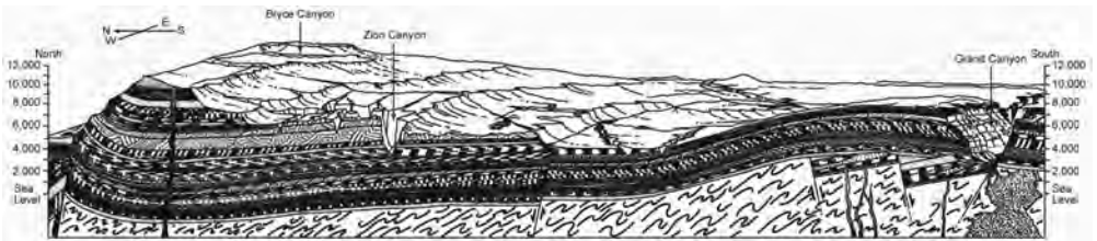
Figure 3. Cross-section through the Grand Canyon-Grand Staircase region showing the extent of the rock layers
